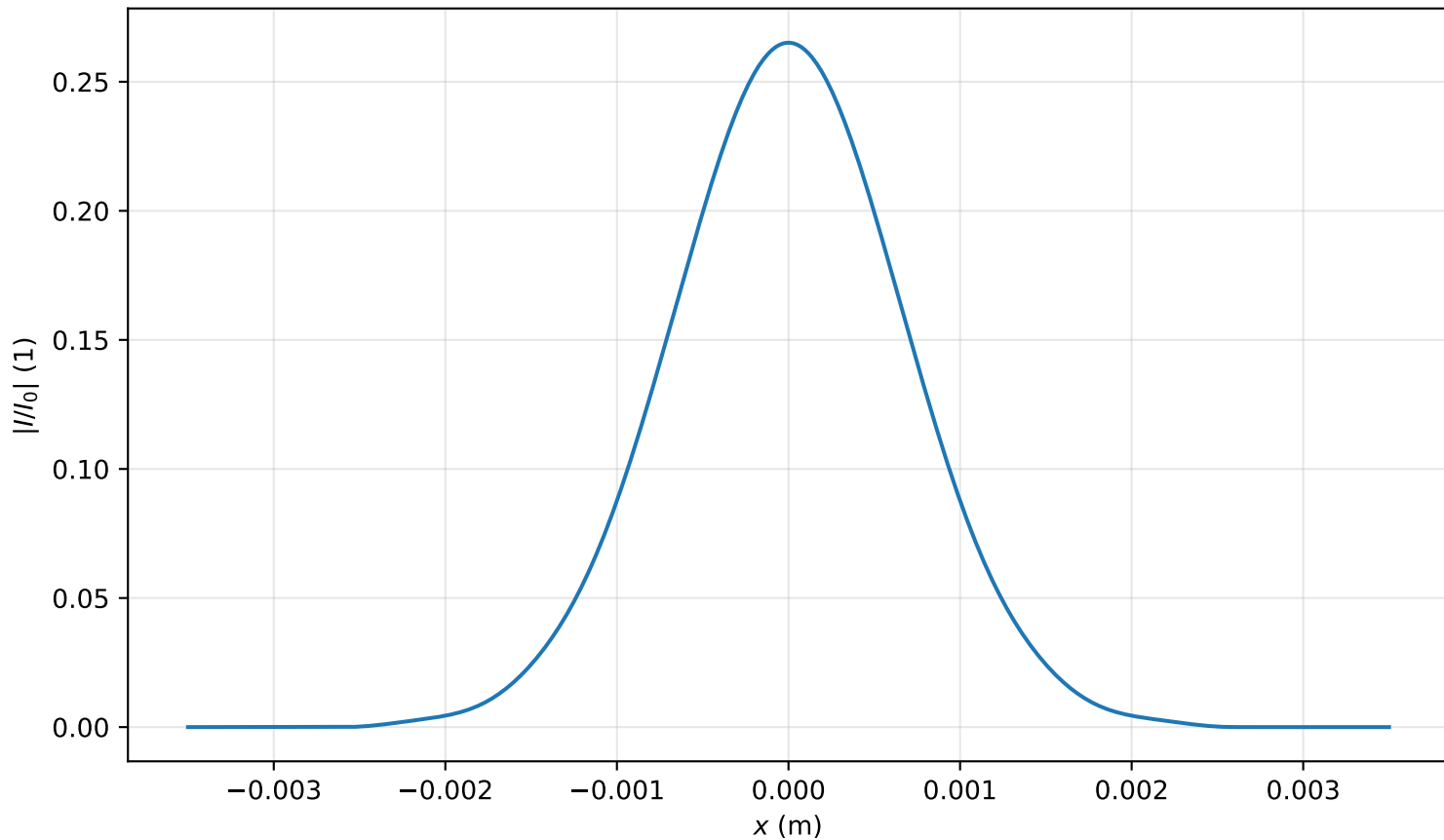
Intensity profile I(x, y = 0, z = 3.821m)/I_0 , P_{in}=0.2P_{cr} , artificial time
